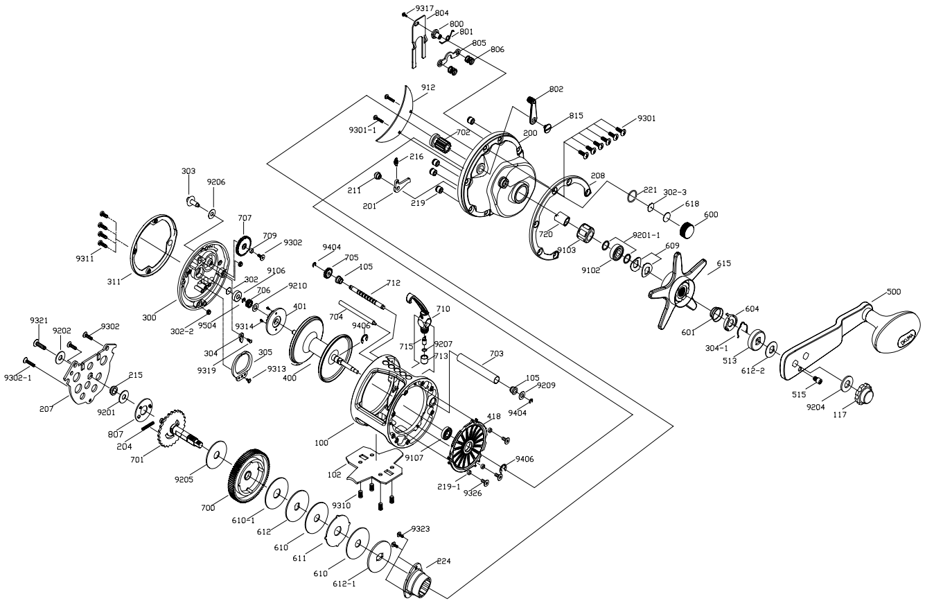
CT - 30L (2 of 2) Spare Parts
